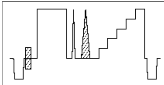
Figure 20. A combination signal that includes a 20T modulated pulse (CCIR Line 17).
