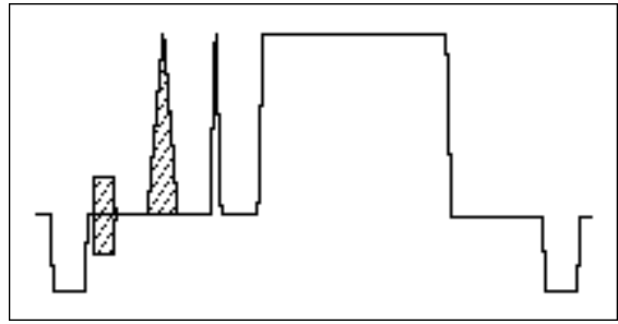
Figure 56. This signal contains the pulse and bar elements required for K Factor measurements.
