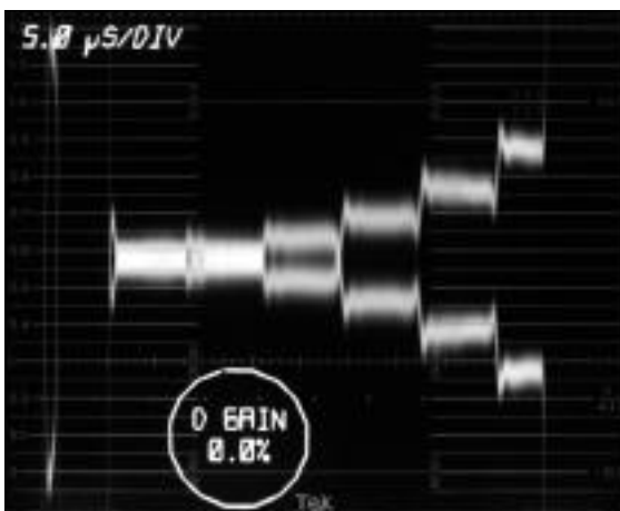
Figure 75. The 1781R double trace DIFF GAIN display with the readout zeroed.
