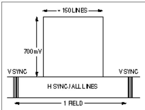
Figure 32. The field square wave test signal.
