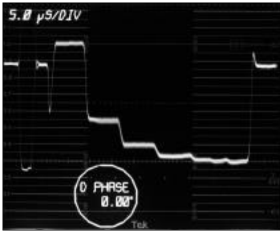
Figure 66. A single trace display indicating about 7 degrees of differential phase distortion.
