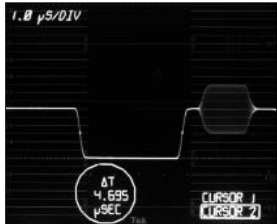
Figure 13. The 1781R time cursors positioned to measure horizontal sync width at the 50% amplitude points.
