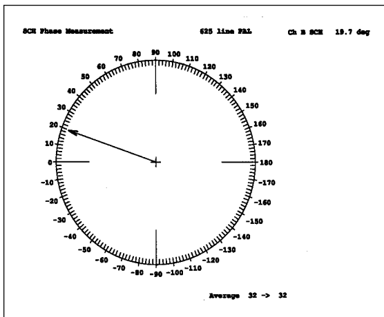
Figure 19. The VM700T SCH Phase Measurement display.
