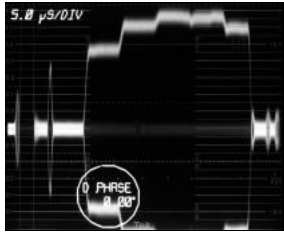
Figure 67. The 1781R double trace DIFF PHASE display with the phase readout zeroed.
