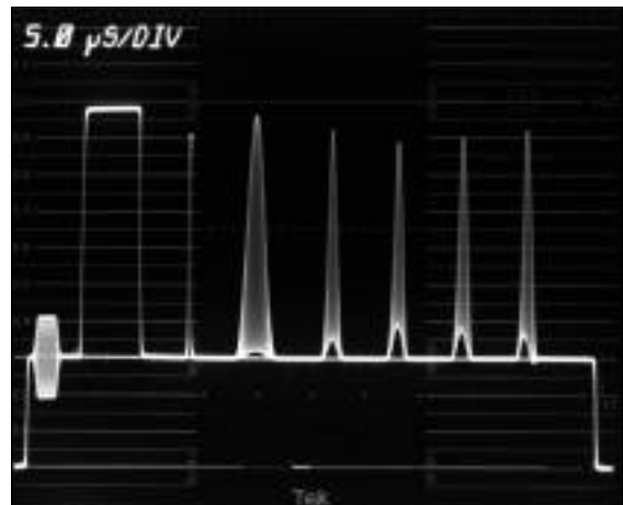
Figure 45. The multipulse signal exhibiting frequency response distortion.
