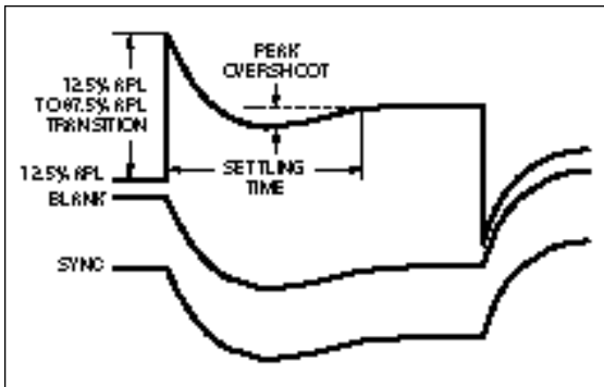
Figure 37. Long time distortion measurement parameters.
