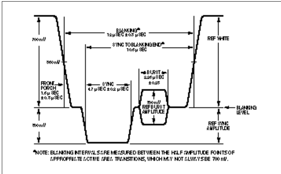
Figure 11. CCIR horizontal pulse width requirements.
