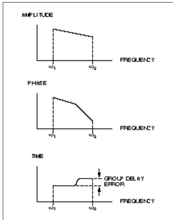
Figure 54. Response of a system with amplitude and phase distortion.
