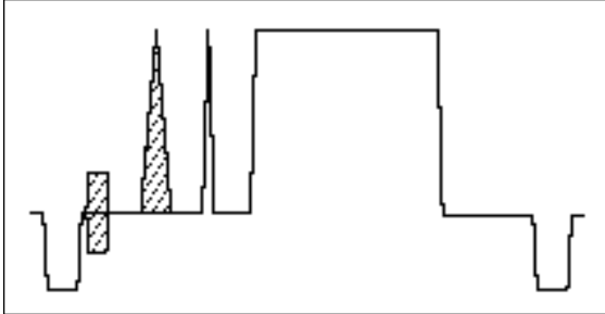
Figure 29. Pulse and bar signal.
