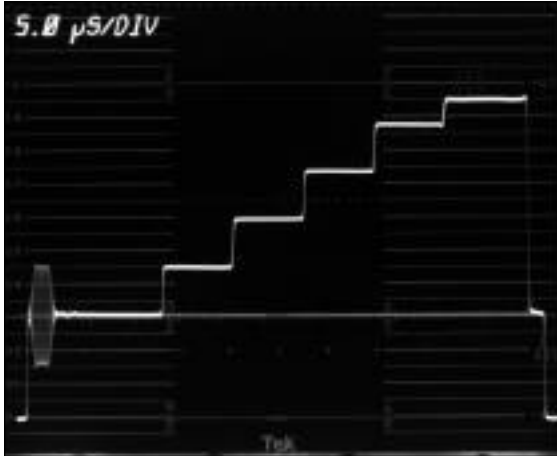
Figure 80. An example of luminance nonlinearity distortion.
