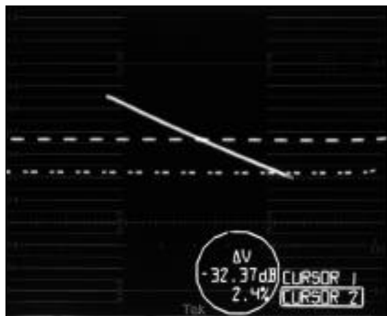
Figure 34. The 1781R voltage cursors can be used to measure field time distortion.
