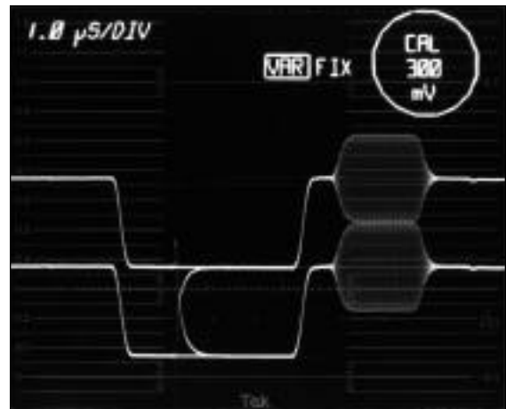
Figure 9. The WFM + CAL mode can also be used to measure sync amplitude.
