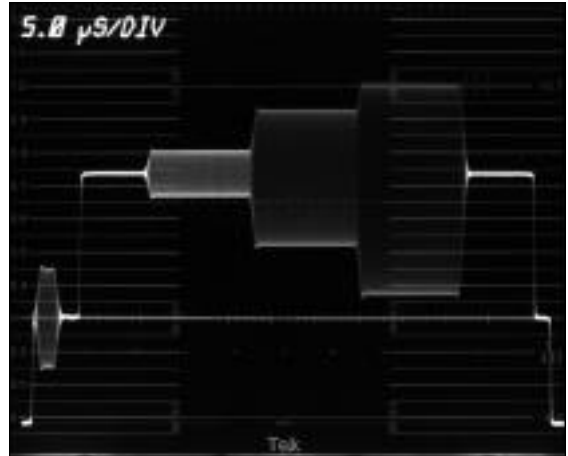
Figure 87. This signal exhibits chrominance nonlinear gain distortion. Note that the amplitude of the largest packet is reduced.
