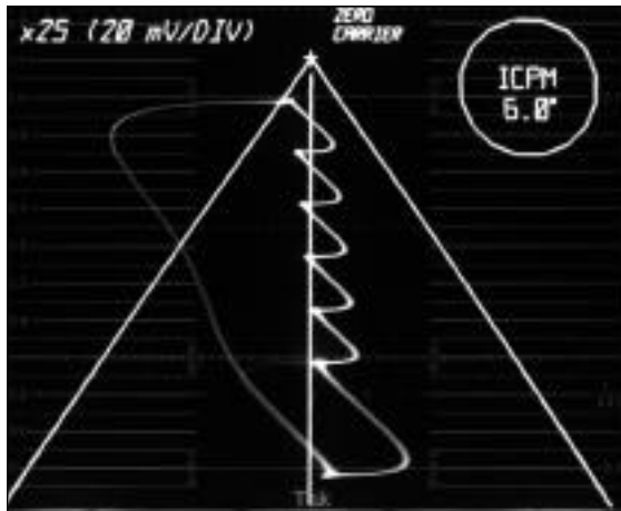
Figure 103. The 1781R electronic graticule indicating an ICPM distortion of 6 degrees.
