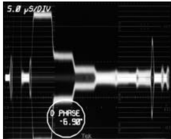
Figure 68. The double trace DIFF PHASE display with the measurement results indicated on the readout.
