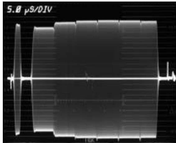
Figure 72. A chrominance filter display indicating about 6% differential gain.
