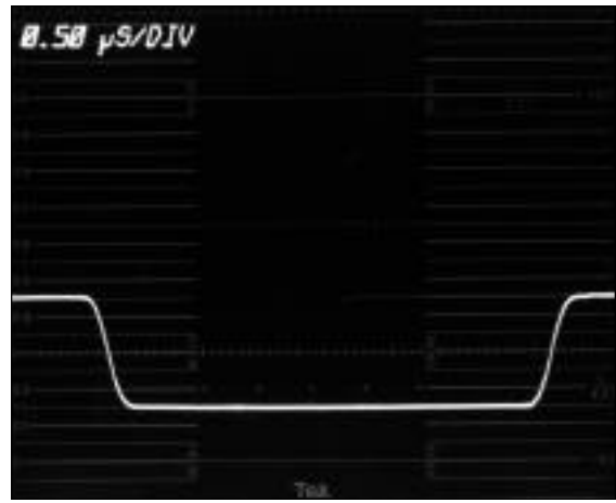
Figure 12. Horizontal sync width measurement at the 50% amplitude points.
