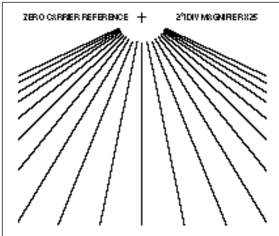
Figure 104. The 1481 ICPM graticule.
