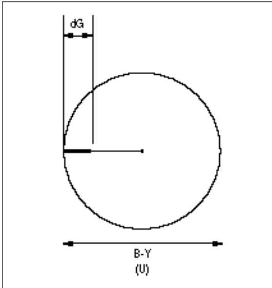
Figure 73. Differential gain distortion affects the B-Y (U) signal.
