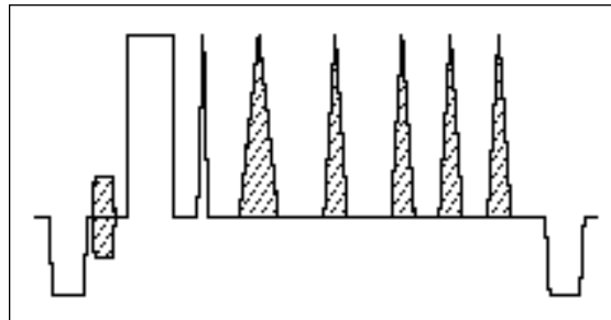
Figure 40. The multipulse test signal.
