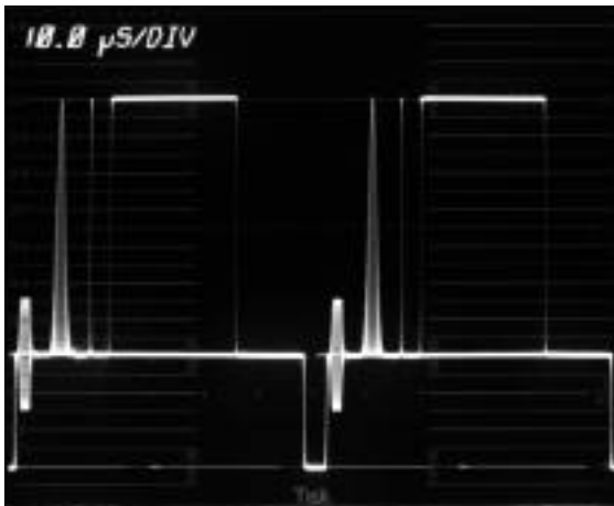
Figure 7. A 1-volt signal properly positioned with respect to the 1781R graticule.
