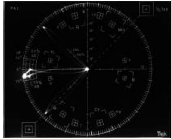
Figure 64. A vectorscope display showing a peak-to-peak differential phase distortion of about 7 degrees. Differential gain distortion is also present.
