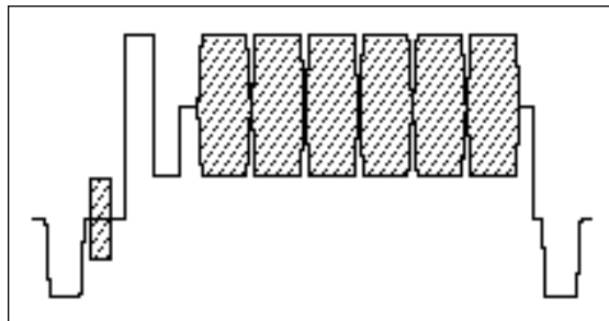
Figure 39. A multiburst test signal.
