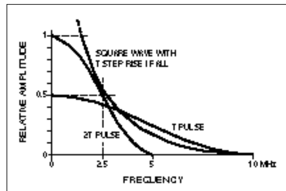
Figure 112. Frequency spectra of T pulse, 2T pulse, and T step.
