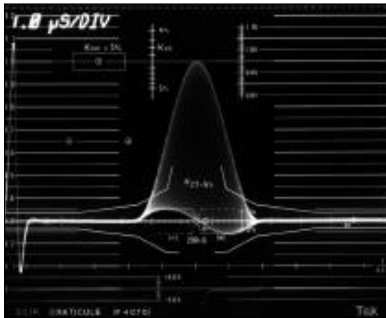
Figure 25. The 1781R graticule indicates that this signal has approximately 200 nanoseconds of chrominance-to-luminance delay.
