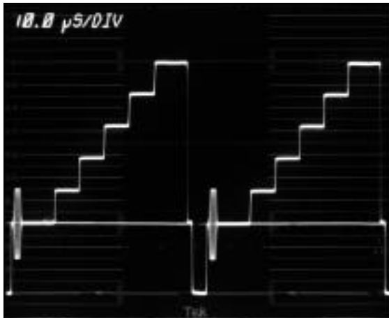
Figure 94. The sync pulse measures 300 mV at 50% APL.
