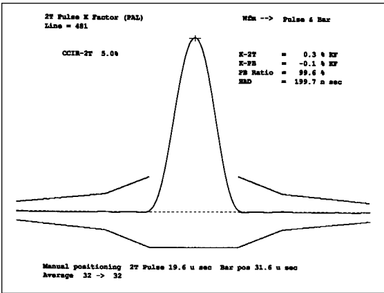
Figure 61. The VM700T 2T Pulse K Factor measurement.
