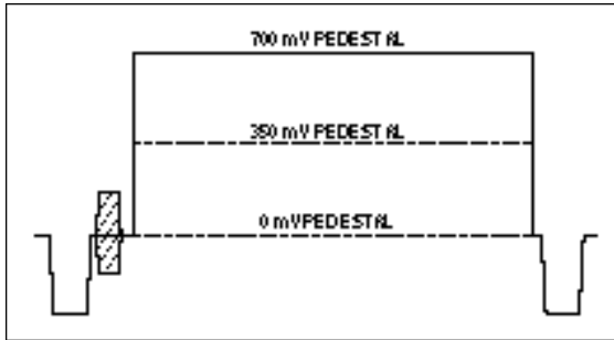
Figure 93. A staircase signal with variable APL.
