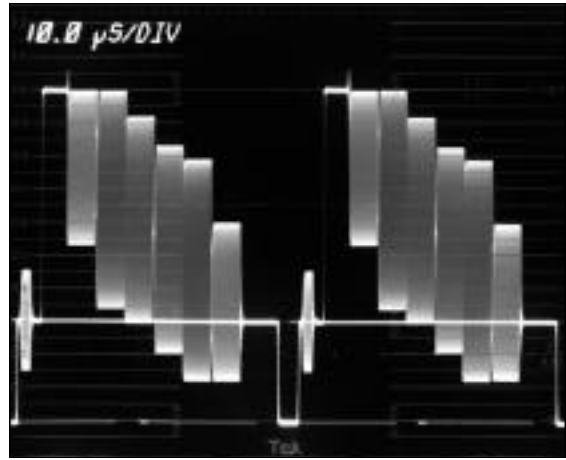
Figure 1. A waveform monitor display of colour bars.
