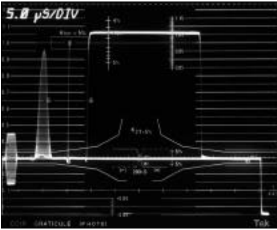
Figure 59. With the pulse taken as the reference, the 1781R graticule indicates that this signal has a K_{\text{pulse/bar}} distortion of 2%.
