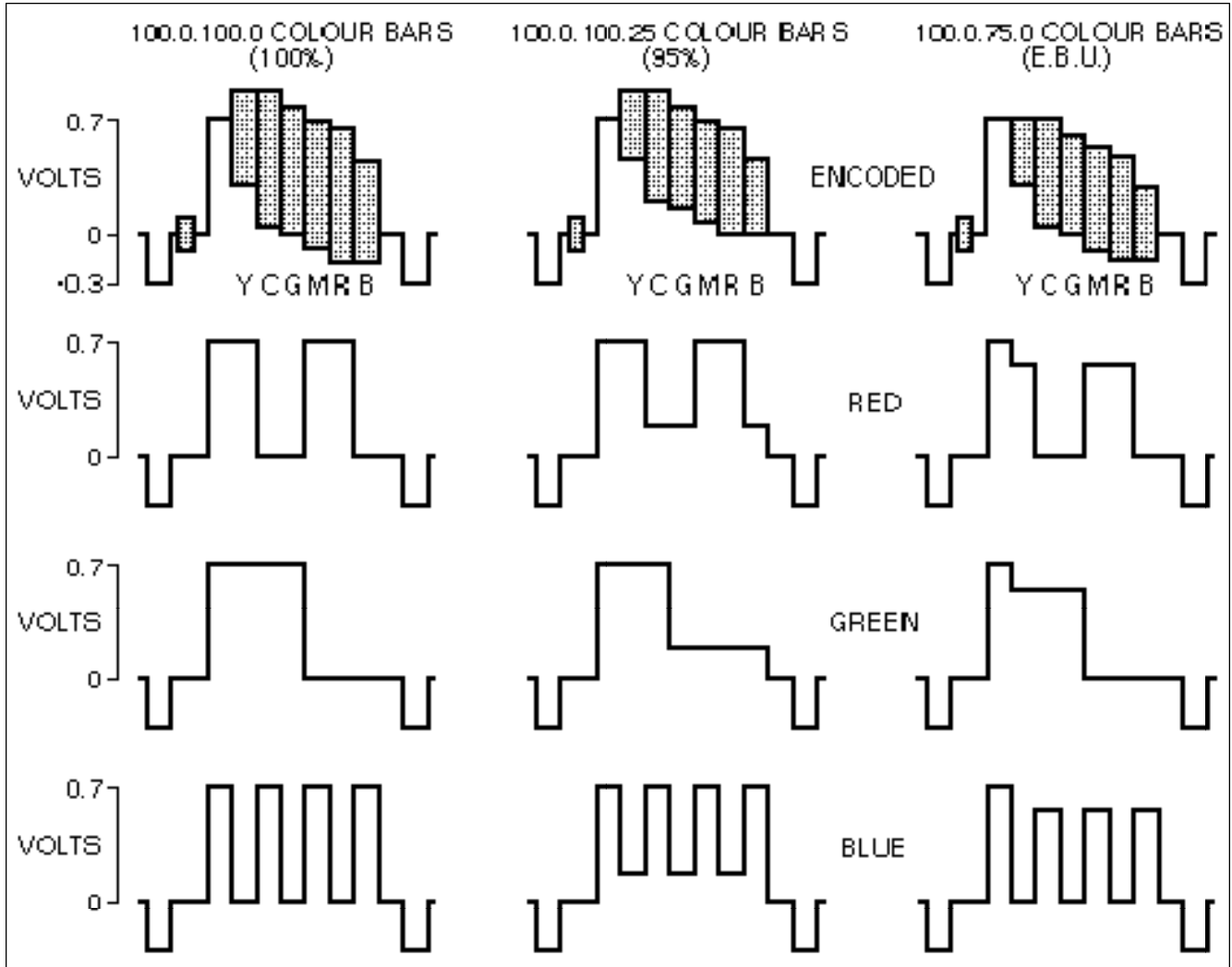
Figure 109. Waveforms and RGB voltages for three types of PAL colour bars.
