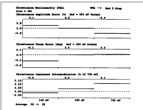
Figure 91. The VM700T Chrominance Nonlinearity display.
