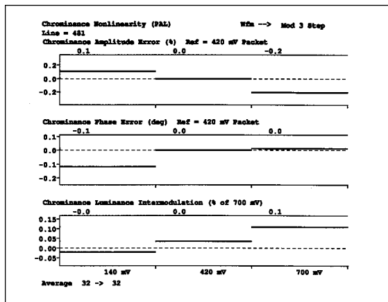
Figure 85. The VM700T Chrominance Nonlinearity display.
