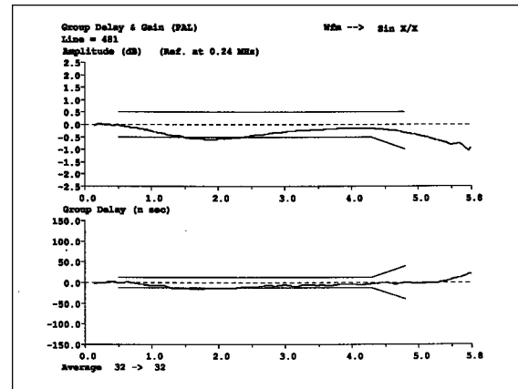
Figure 49. The VM700T Group Delay & Gain measurement made with the (sin x)/x signal.
