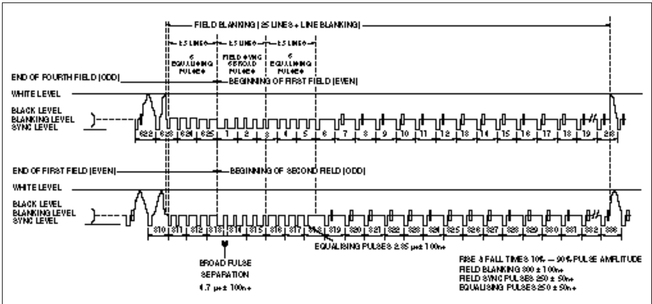
Figure 17. CCIR vertical interval specifications.
