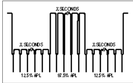
Figure 92. A flat field bounce test signal.
