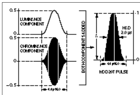
Figure 21. The chrominance and luminance components of a modulated sine-squared pulse.
