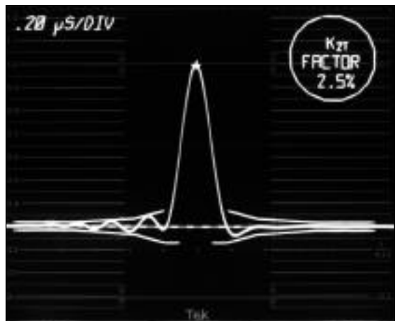
Figure 58. The 1781R electronic K Factor graticule measures a 2.5% K_{2T} distortion for this signal.
