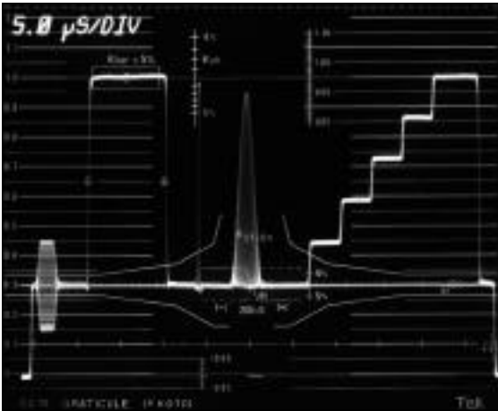
Figure 60. This signal is properly positioned for a K_{\text{bar}} measurement with the 1781R graticule.
