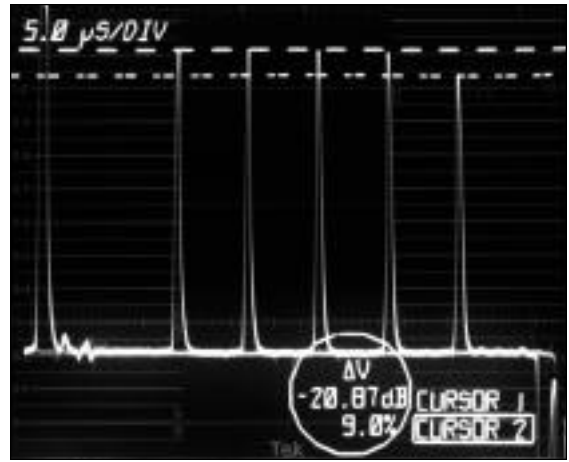
Figure 81. This photograph shows a 5 step staircase after it has been passed through a differentiated step filter. The 1781R voltage cursors indicate 9% luminance nonlinearity.
