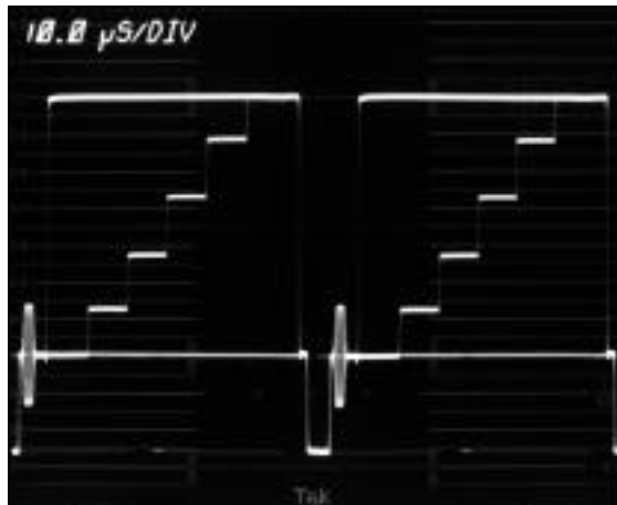
Figure 95. At 87.5 APL, the sync pulse measures 260 mV. This indicates a steady-state distortion of about 13%.
