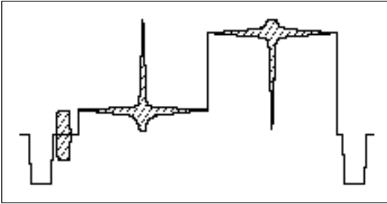
Figure 42. A time domain display of the (\sin x)/x signal.
