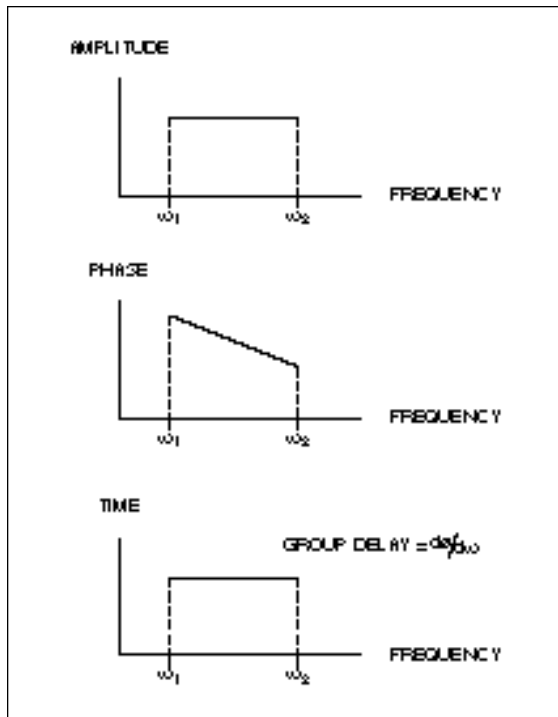
Figure 53. Response of a distortion free system.
