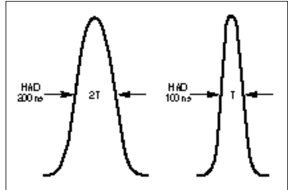
Figure 110. 2T pulse and 1T pulses for PAL systems.
