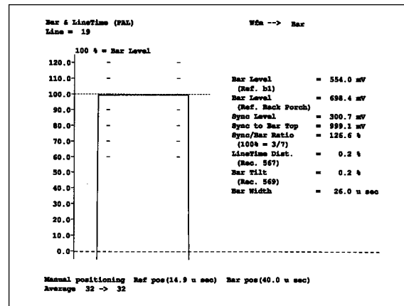
Figure 31. The VM700T Bar Line Time display.
