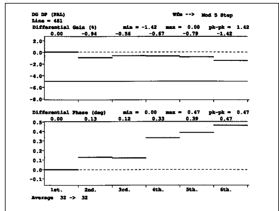
Figure 69. The VM700T DG DP display.
