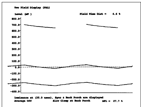
Figure 35. The VM700T Two Field display.
