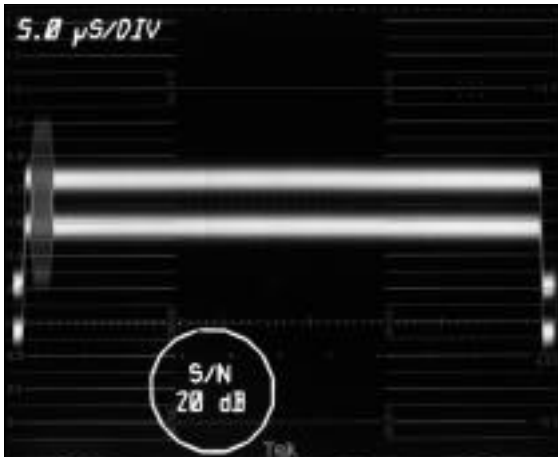
Figure 97. The 1781R tangential noise measurement mode showing excessive trace separation.
