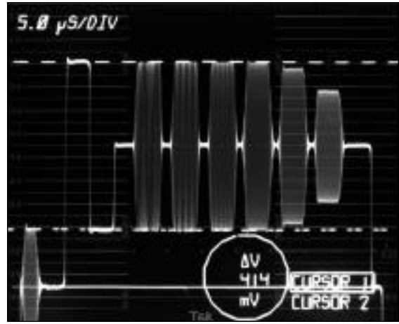
Figure 43. The low-frequency square wave is defined as the reference.
