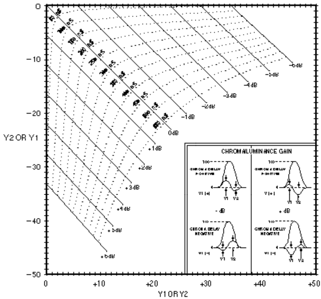
Figure 23. Chrominance-to-luminance gain and delay nomograph for a 20T pulse.
