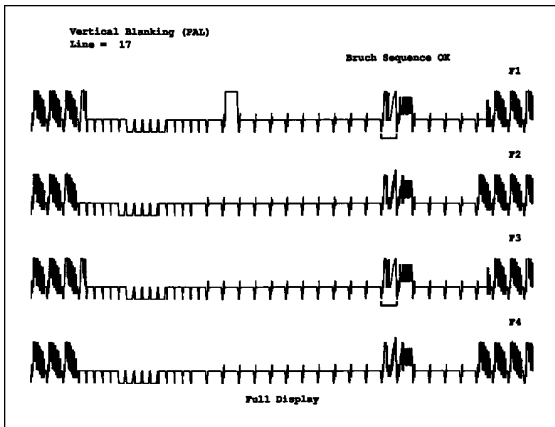
Figure 16 The VM700T Vertical Blanking display.
