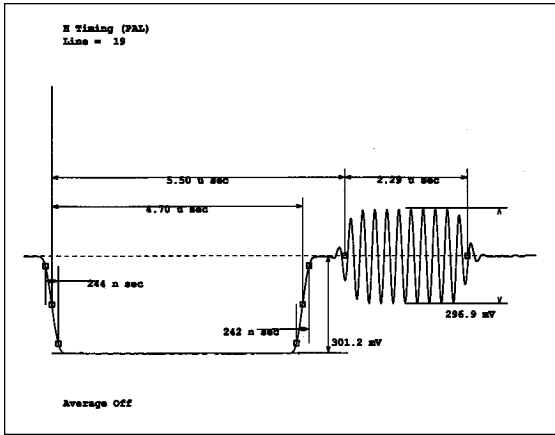
Figure 15. The VM700T H Timing display.
