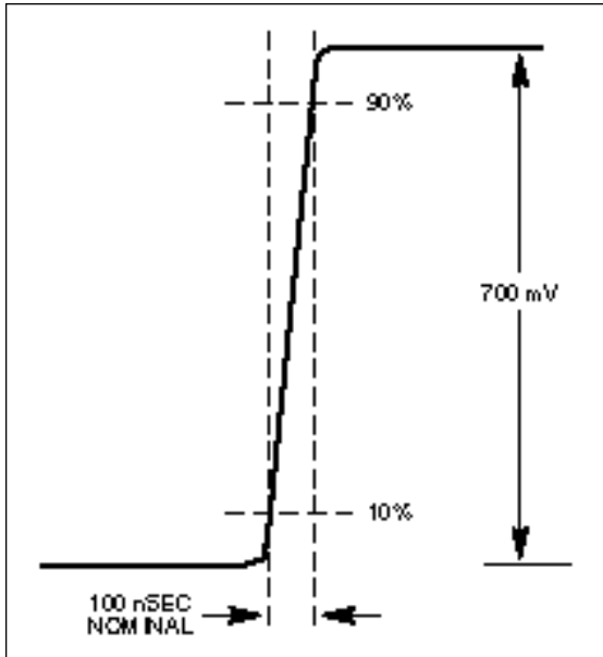
Figure 27. A T rise time bar has a 10% to 90% rise time of nominally 100 nanoseconds.
