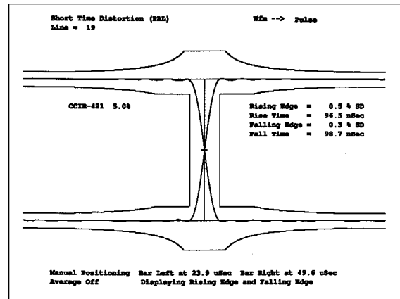
Figure 28. The VM700T Short Time Distortion display.
