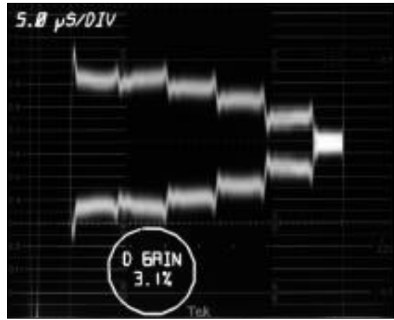
Figure 76. The 1781R double trace DIFF GAIN display showing measurement results. With attenuation only, peak and peak-to-peak results are the same.
