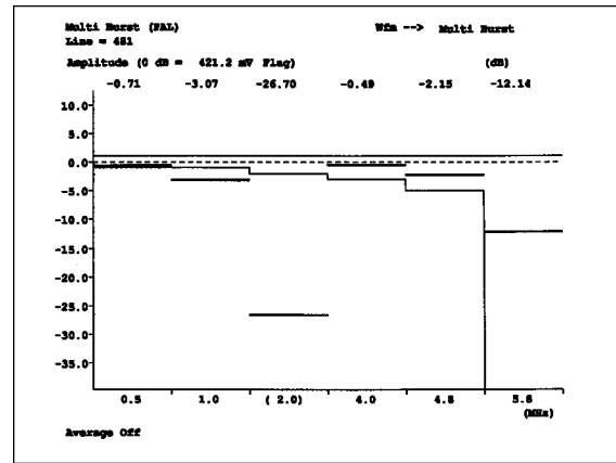
Figure 48. The VM700T Multiburst measurement.
