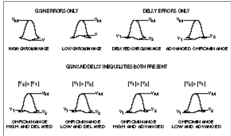
Figure 22. Effects of gain and delay inequalities on the modulated sine-squared pulse.
