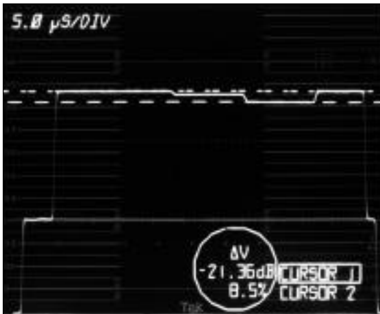
Figure 90. A chrominance-to-luminance intermodulation distortion of 8.5% referenced to the pedestal level.
