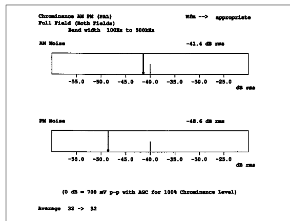
Figure 100. The VM700T Chrominance AM PM display.
