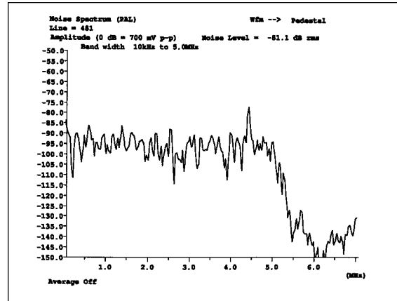
Figure 99. The VM700T Noise Spectrum display.
