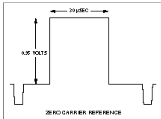
Figure 107. The zero carrier reference pulse as it appears in a baseband signal (System I).
