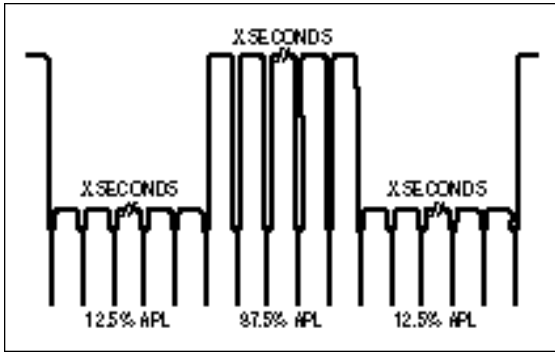
Figure 36. A flat field bounce signal.
