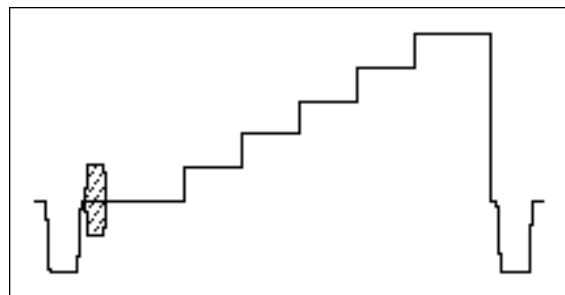
Figure 108. A signal that extends to 700 mV, such as this staircase signal, is used in conjunction with the zero carrier pulse to verify modulation levels.
