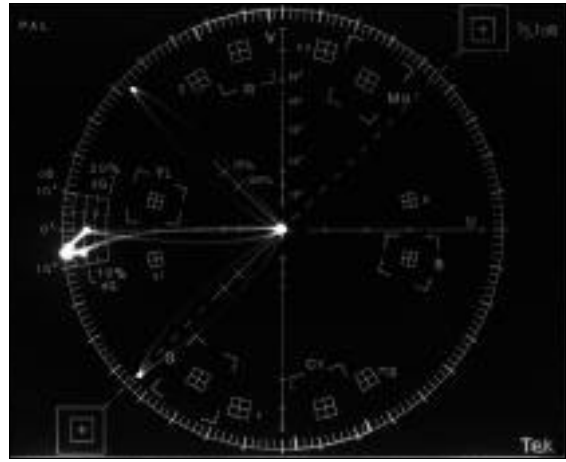
Figure 71. A vectorscope display of a signal with 10% peak-to-peak differential gain. Differential phase distortion is also present.
