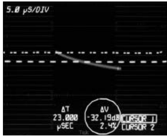
Figure 30. The 1781R voltage and time cursors can facilitate line time distortion measurements.
