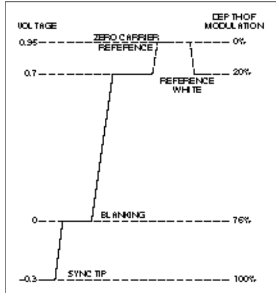
Figure 106. Depth of modulation levels for System I.
