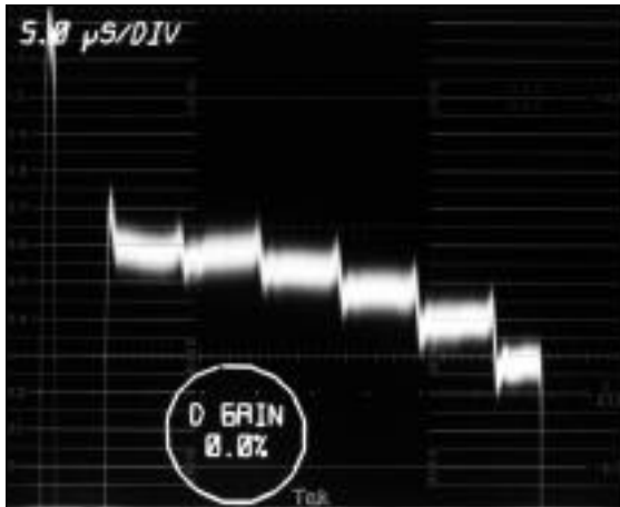
Figure 74. A single trace DIFF GAIN display indicating a distortion of about 3%.
