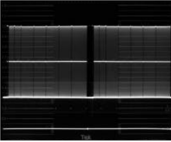
Figure 41. A 6 MHz field-rate sweep signal with markers (2-field display).
