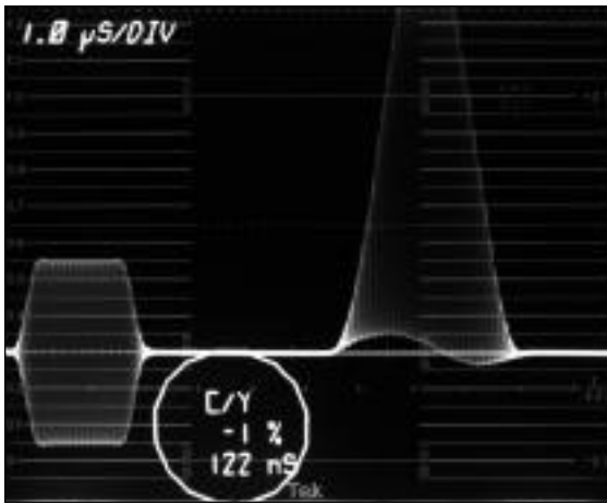
Figure 24. Results obtained with the CHROMA/LUMA selection in the 1781R MEASURE mode.
