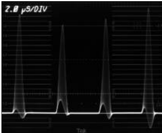
Figure 51. The multipulse signal exhibiting group delay distortion. Group delay differences between the high frequency and low frequency components of the pulse appear as sinusoidal distortion of the baseline.
