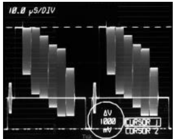
Figure 10. 1781R voltage cursors positioned to measure peak-to-peak amplitude.
