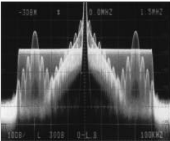
Figure 47. A spectrum analyzer display of a (\sin x)/x signal with a cutoff frequency of 6 MHz.
