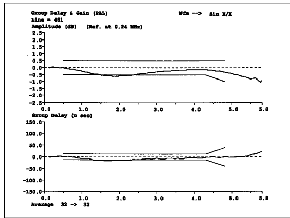
Figure 52. The VM700T Group Delay & Gain measurement made with the (\sin x)/x signal.
