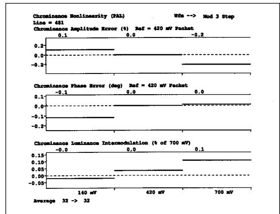
Figure 88. The VM700T Chrominance Nonlinearity display.
