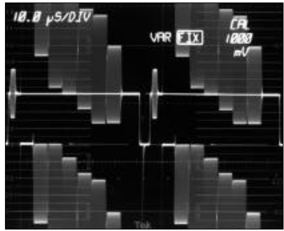
Figure 8. The WFM + CAL mode in the 1781R indicates that insertion gain is properly adjusted.
