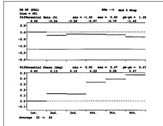
Figure 77. The VM700T DG DP display.
