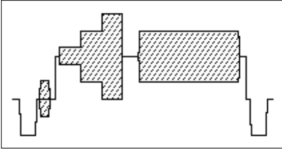
Figure 89. This combination ITS contains the Modulated Pedestal signal element (CCIR Line 331).
