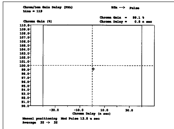
Figure 26. The Chrom/Lum Gain Delay display in the VM700T MEASURE mode.
