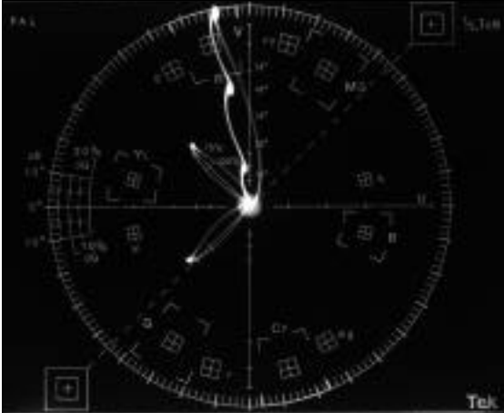
Figure 84. The 1781R vectorscope display showing a signal that suffers from chrominance nonlinear phase distortion.
