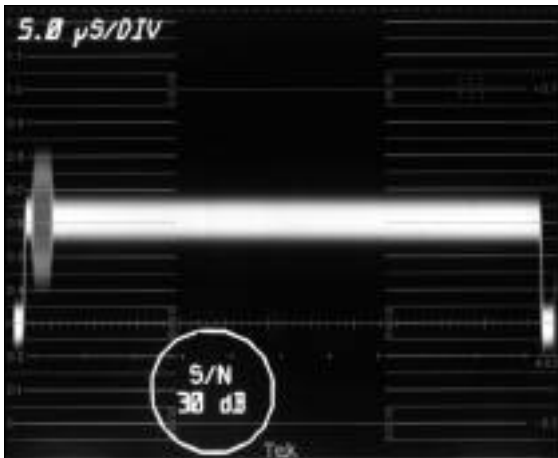
Figure 98. The 1781R tangential noise measurement mode with trace separation properly adjusted. This signal has a signal-to-noise ratio of 30 dB.
