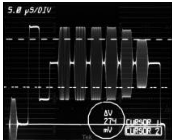
Figure 44. The peak-to-peak amplitude of the smallest packet is then measured.
